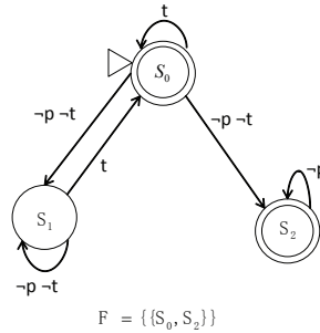
Fig. 1. A general Büchi automaton representing the LTL property \mathbf{G}(\neg t \Rightarrow ((\neg p \mathbf{U} t) \vee \mathbf{G}\neg p)) .
